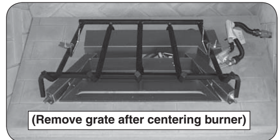
Fig. 19-4 Position grate
