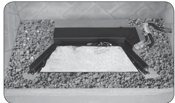
Fig. 20-3 Place sand/vermiculite
