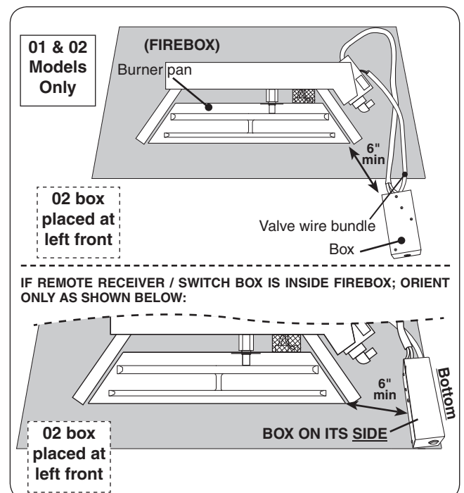
Fig. 18-3 Switch box placement (if applicable)
